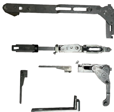
Roto Transmission Box For Tilt & Turn, Lock Set, Corner Connector
